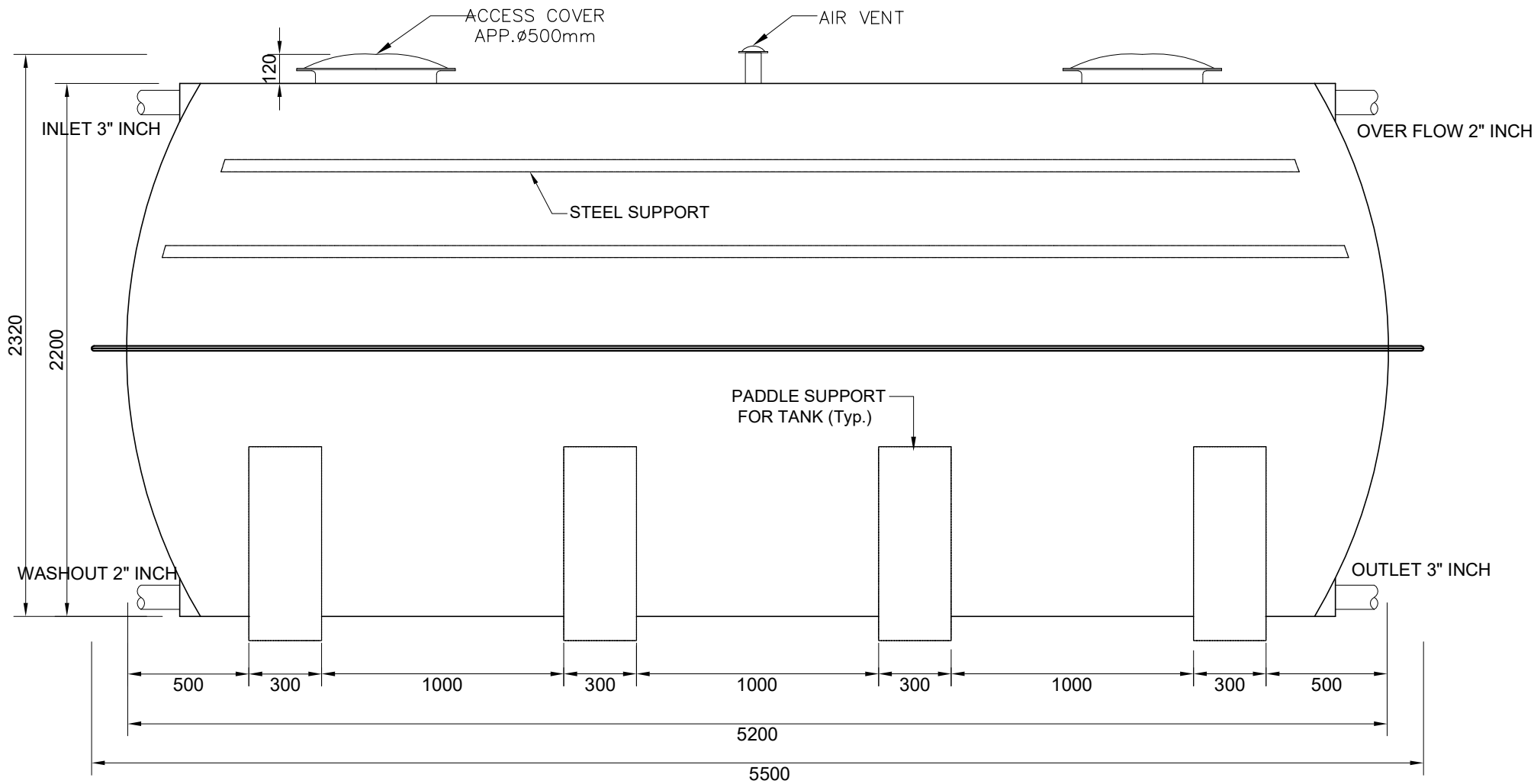
ELEVATION VIEW
