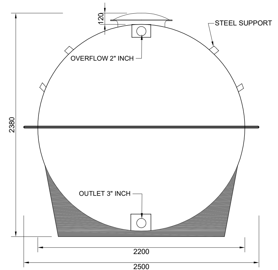
SECTION VIEW
